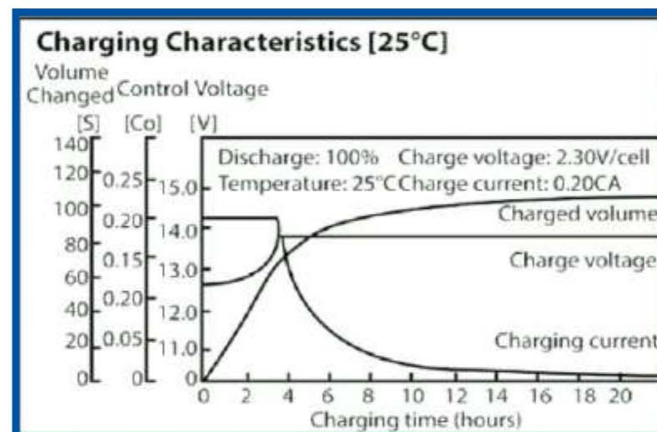
Charging Characteristics
