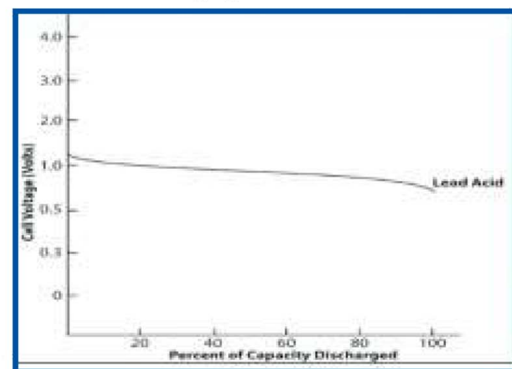
Discharging Characteristics
